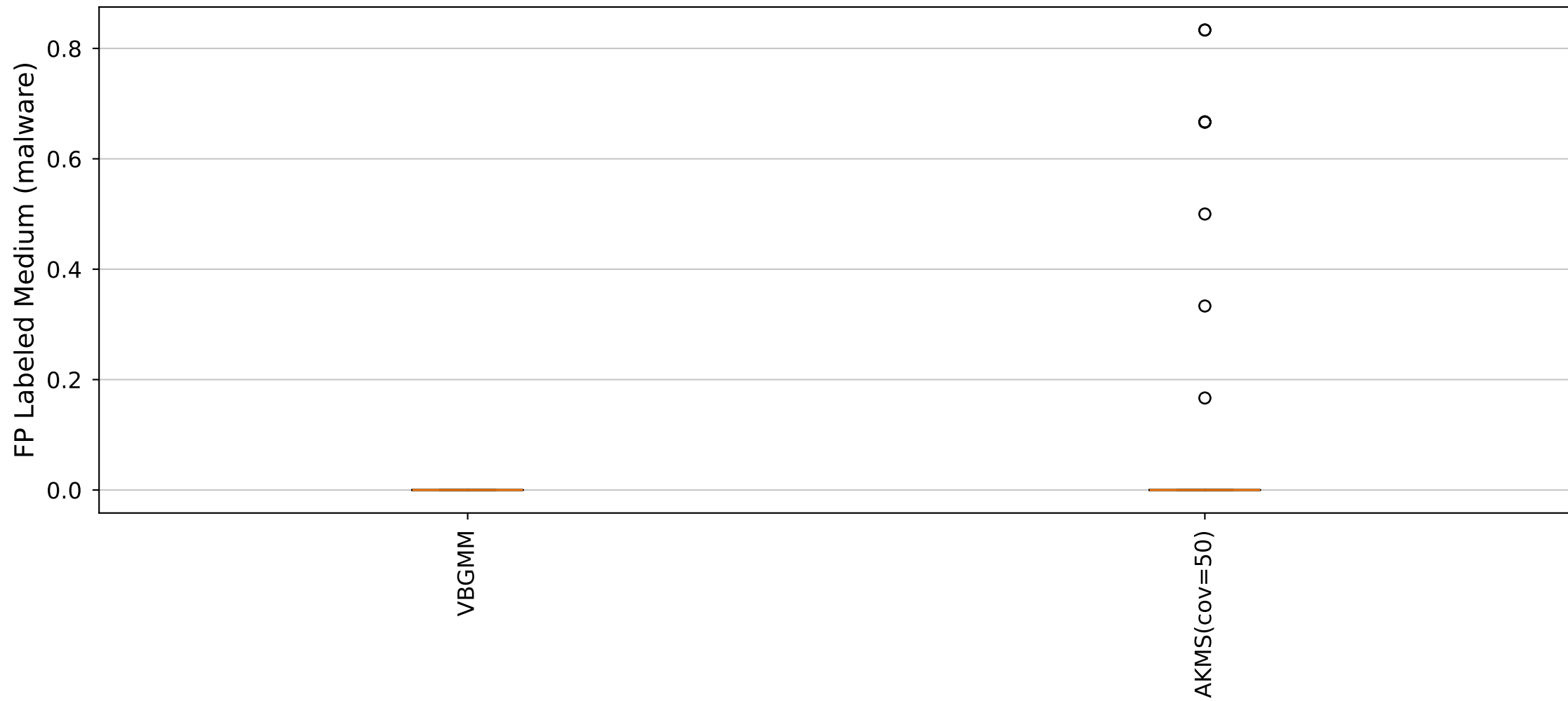
YARA Rules FP Labeled Medium (malware) Distribution (Cluster3_Size53 dataset)
